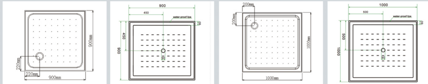
SQUARE 800/900/1000mm
