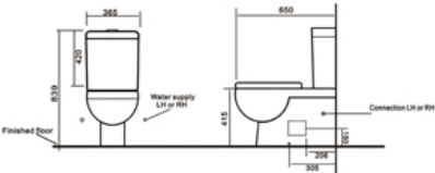
A3209 Back To Wall S PAN: 110-190mm set out P PAN: 180mm set out
