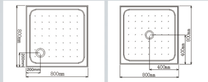
SQUARE 800/900/1000mm
