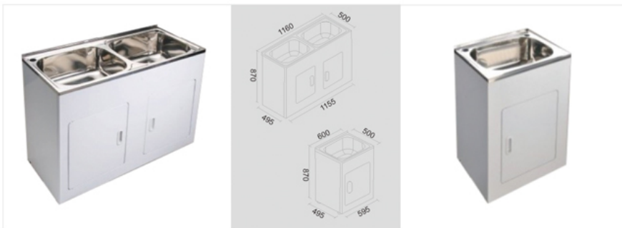
DB652B (Twins45L)+Cabinet Size:1160x500x870mm
