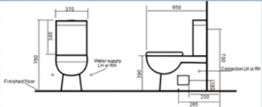
A3958 Back To Wall S PAN: 110-190mm set out P PAN: 180mm set out
