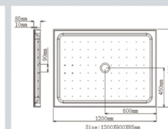
Size: 1200X900X85mm
